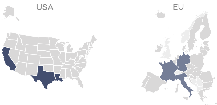
Top regional industrial greenhouse gas emitters in 2021
